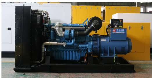
OPEN TYPE
